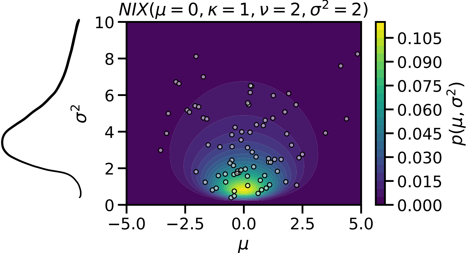
Figure: The NIX(\mu_0, \kappa_0, \nu_0, \sigma_0^2) pdf. Note the dependence: large values of \sigma^2 imply larger variance in p(\mu | \sigma^2) .
